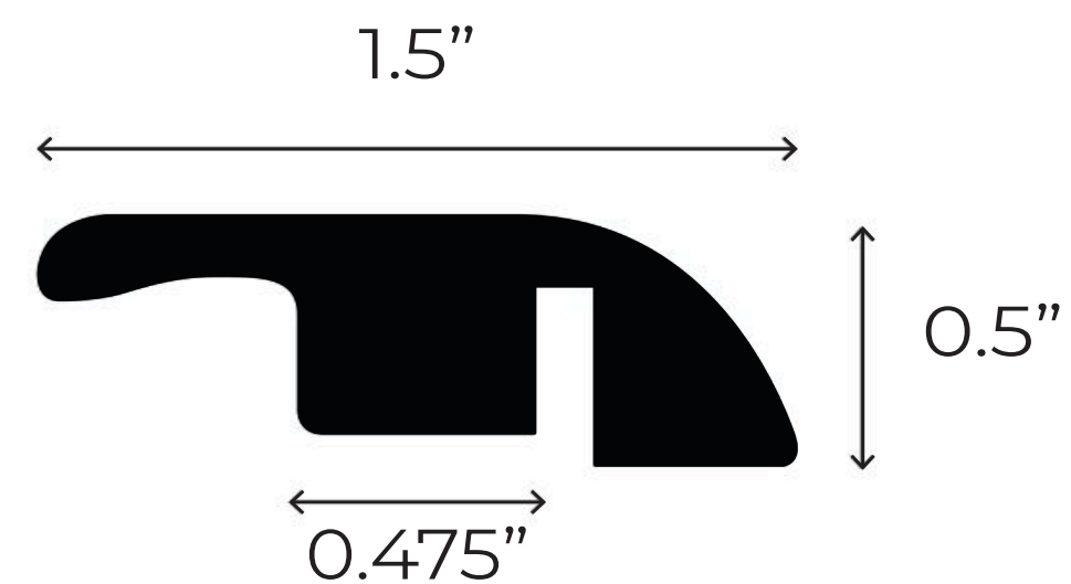
SURFACE REDUCER
